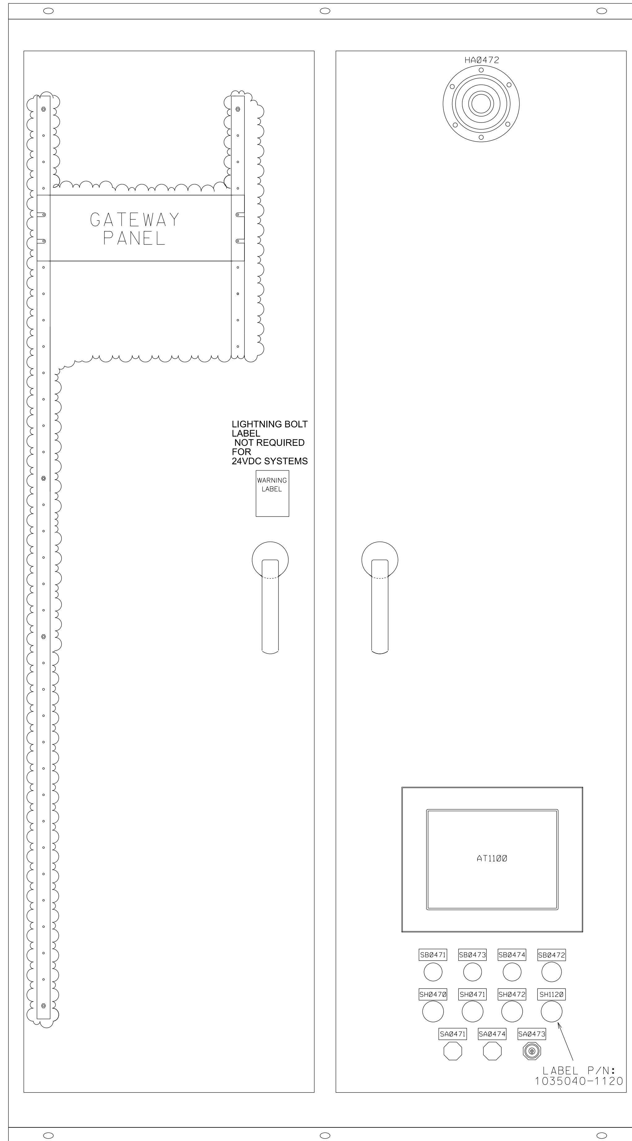
FRONT VIEW
